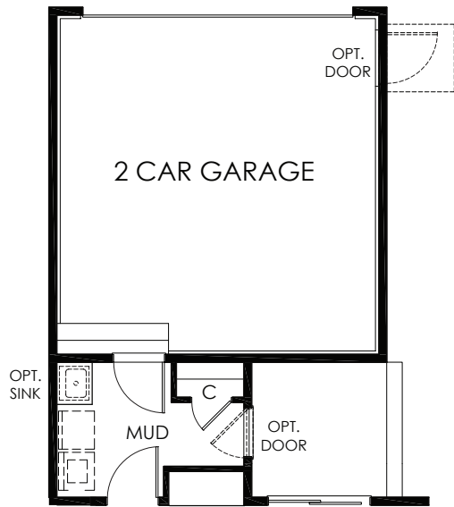
Optional Attached Garage and Mud Room
